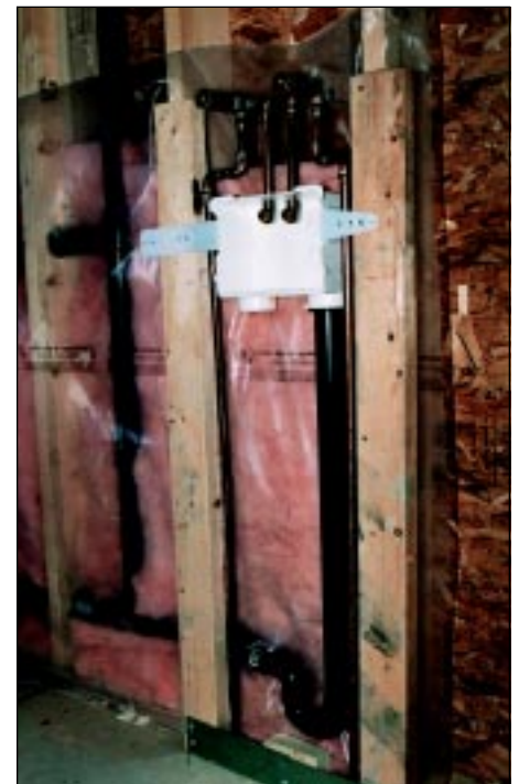
Copper tube and fittings used for a laundry tub and clothes washer.
